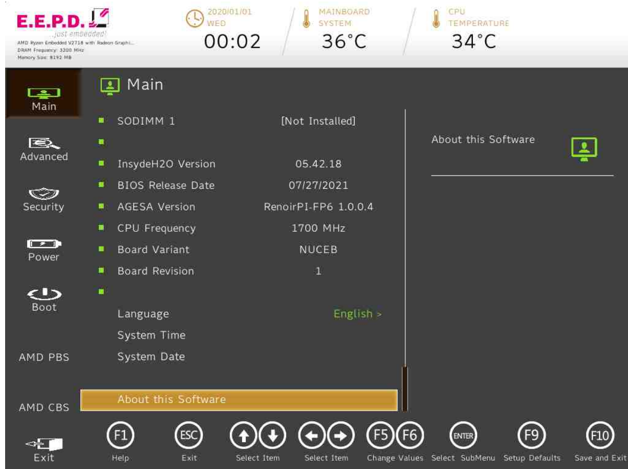
Fig. 17: Main Menu 2
