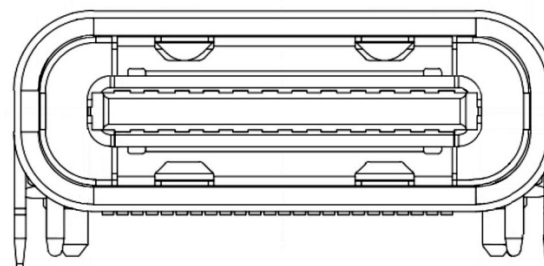
Fig. 15: USB-C 3.1 Gen2 Detail
